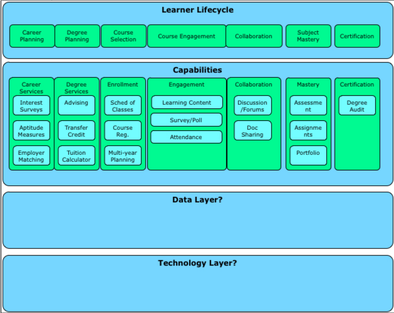
Role Based Lifecycle Reference Architecture Model
